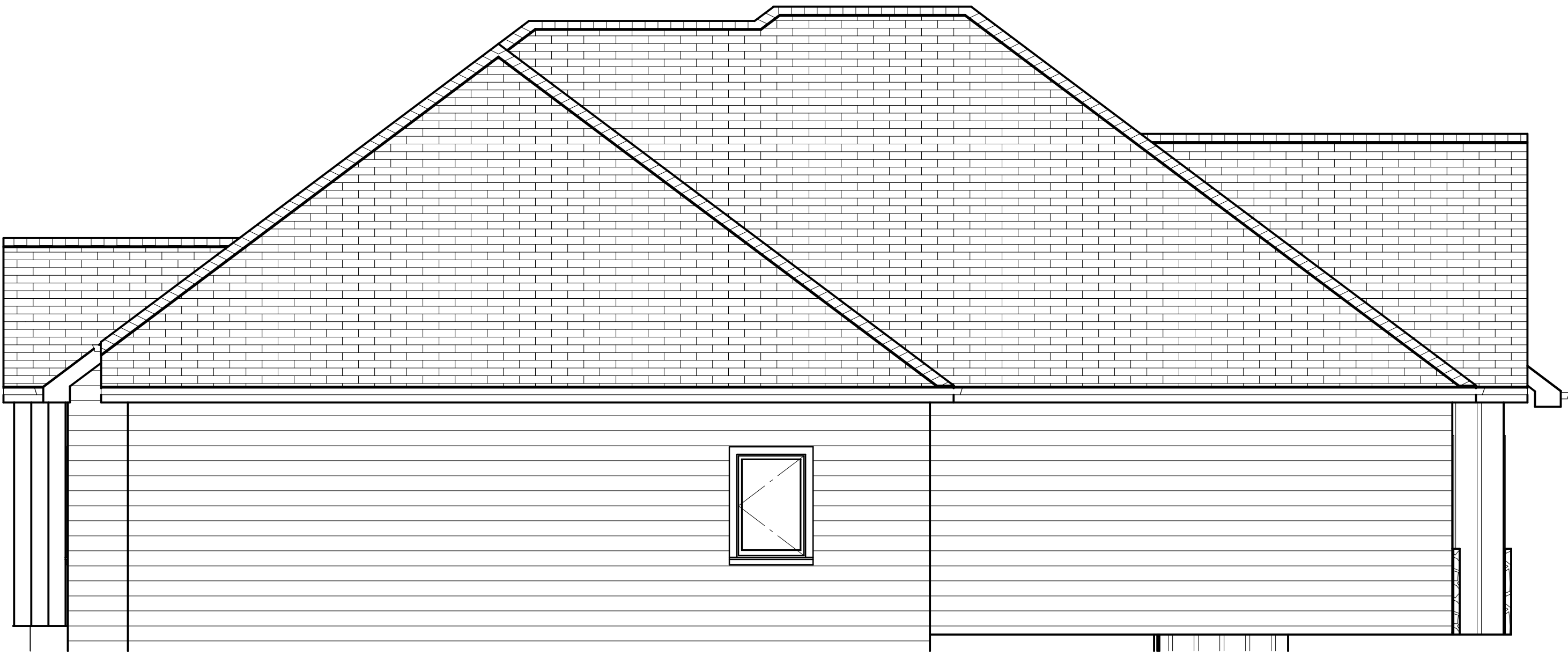
E4 EXTERIOR ELEVATION RIGHT 1/4 IN = 1 FT
