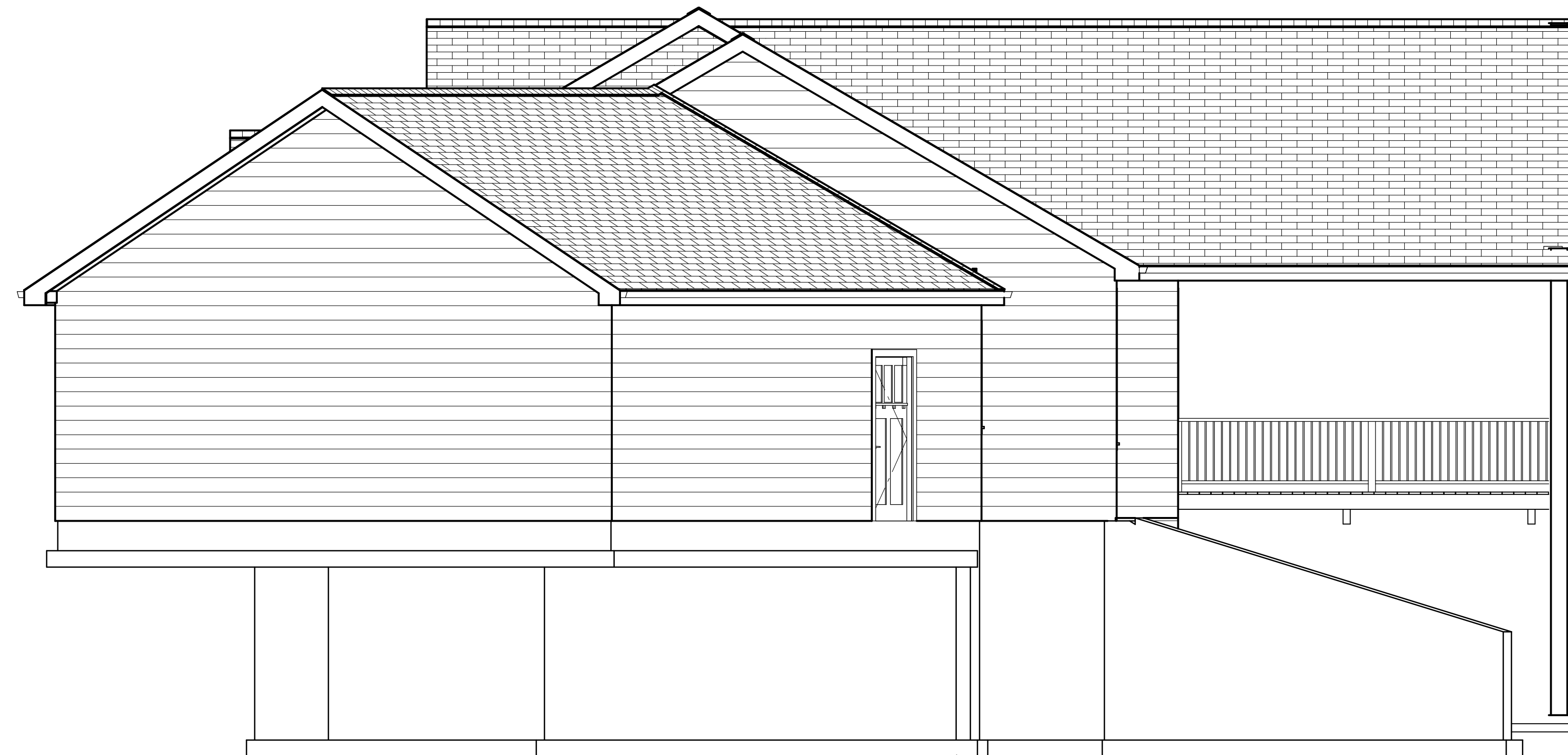
E4 EXTERIOR ELEVATION RIGHT 1/4 IN = 1 FT
