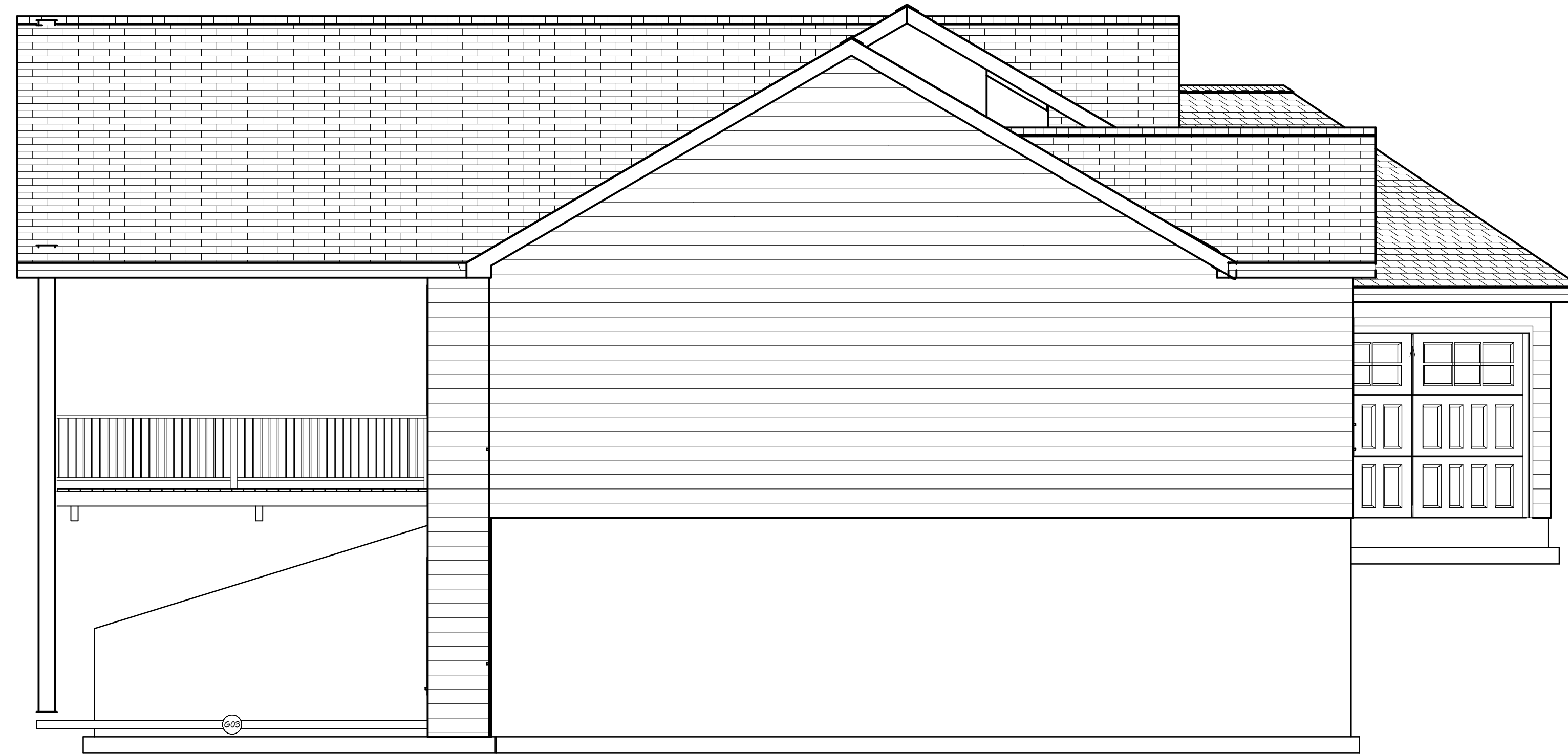
E2 EXTERIOR ELEVATION LEFT 1/4 IN = 1 FT
