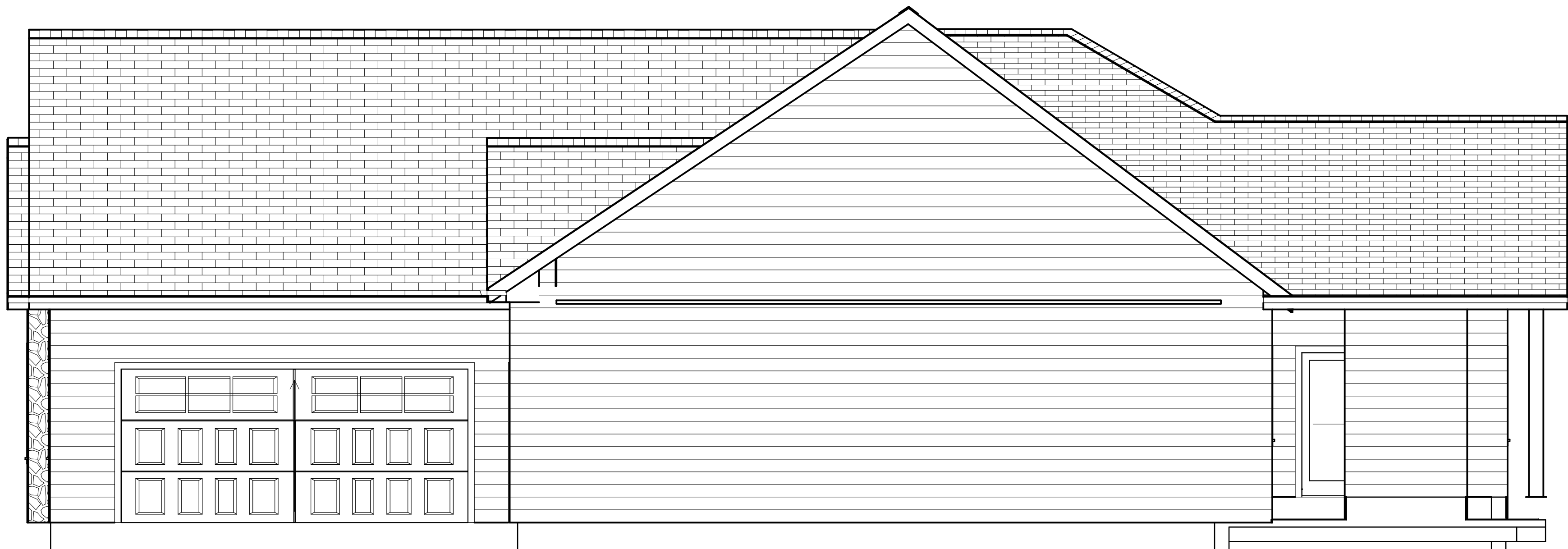
E4 EXTERIOR ELEVATION RIGHT 1/4 IN = 1 FT
