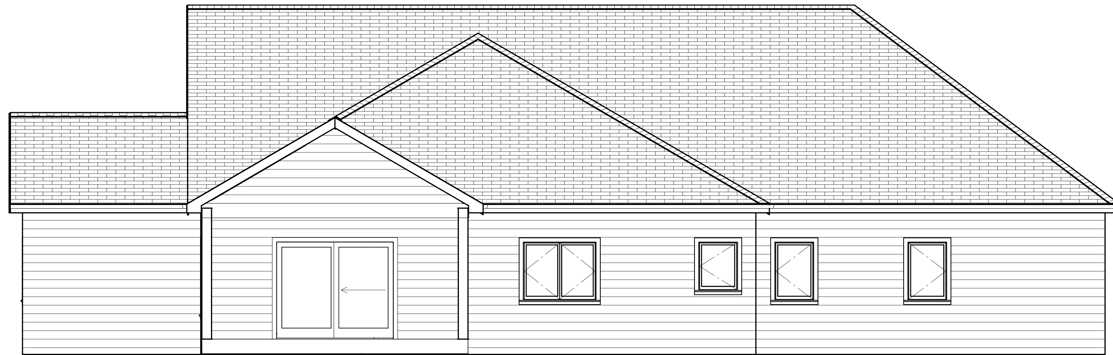
E3 EXTERIOR ELEVATION BACK 1/4 IN = 1 FT
