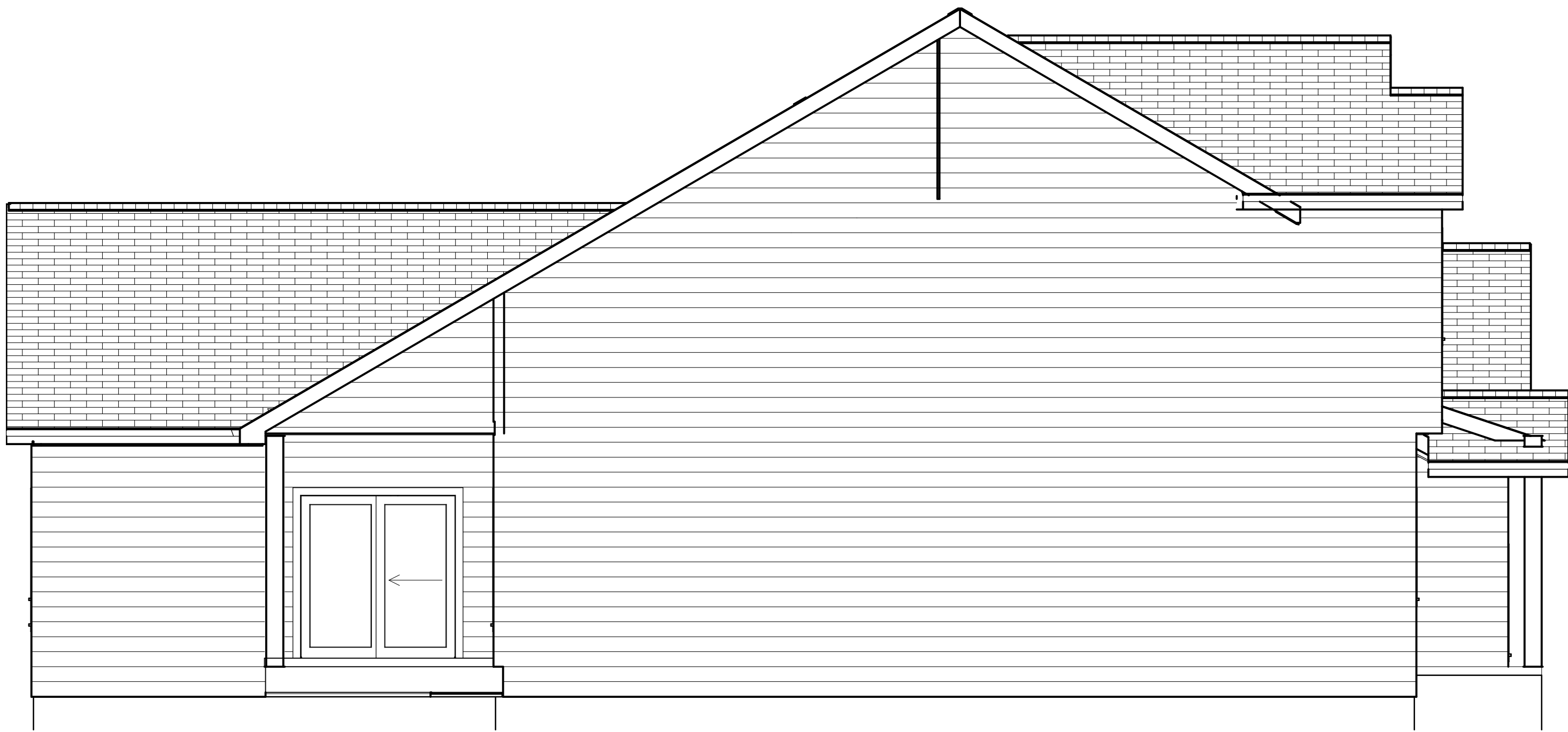
E4 EXTERIOR ELEVATION RIGHT 1/4 IN = 1 FT
